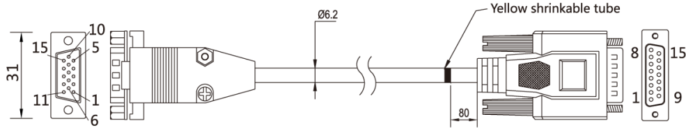
Three-row 15 pin DB female Motor side
