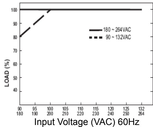
Static Characteristics
