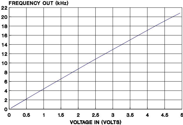
VCO IN vs. Frequency Out High Speed Range
